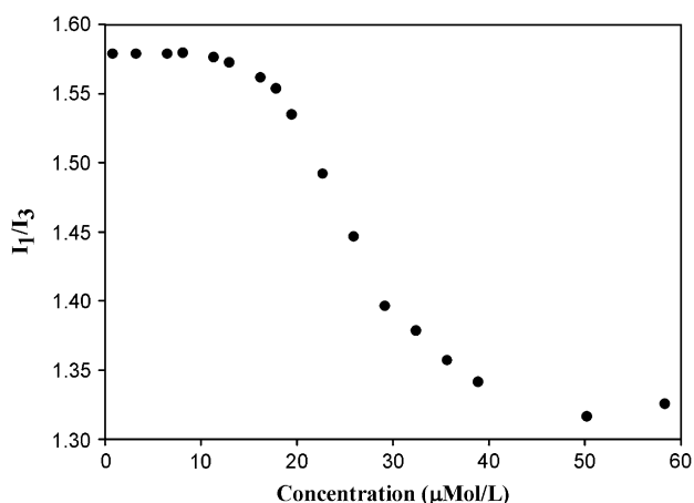
Fig. 4. Plot of the fluorescence pyrene I_1/I_3 intensity ratio vs. concentration data for 16-3-16 2Br.
