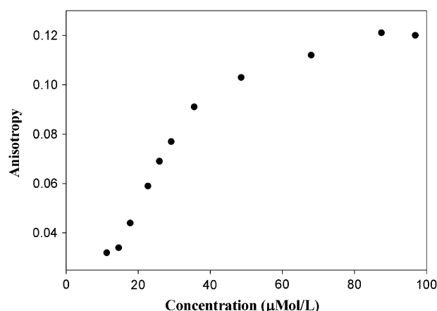
Fig. 5. Plot of the fluorescence anisotropy of fluorescein sodium salt vs. concentration for 16-3-16 2Br.
