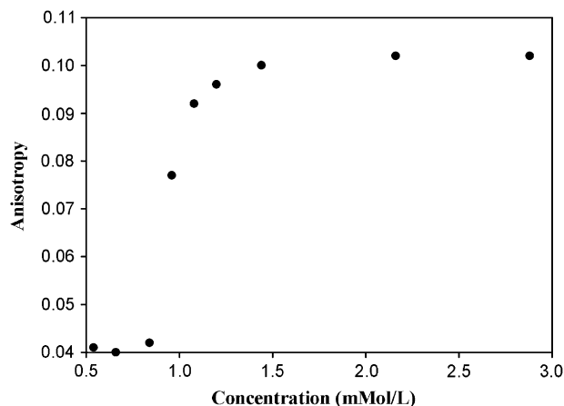
Fig. 6. Plot of the fluorescence anisotropy of fluorescein sodium salt vs. concentration for CTAB.
