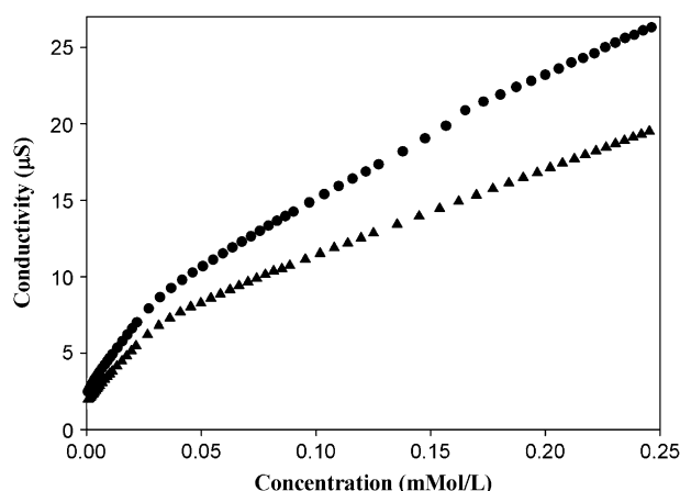
Fig. 2. Plot of conductivity vs. concentration for • 16-3-16 2Br and ▲ 16-4-16 2Br.
