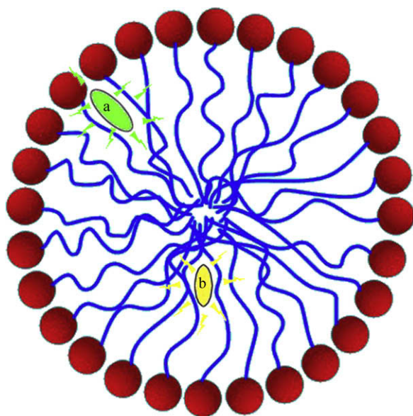
Fig. 7. Pictorial view of the different fluorophores location in the micelle: (a) fluorescein sodium salt near the headgroups, (b) perylene near the core.
