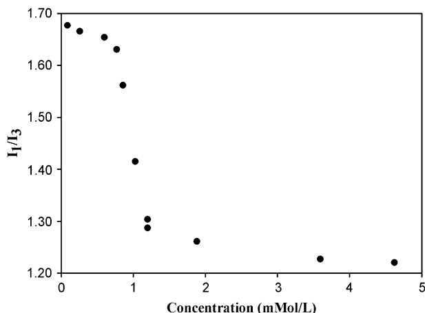
Fig. 3. Plot of the fluorescence pyrene I_1/I_3 intensity ratio vs. concentration data for CTAB.
